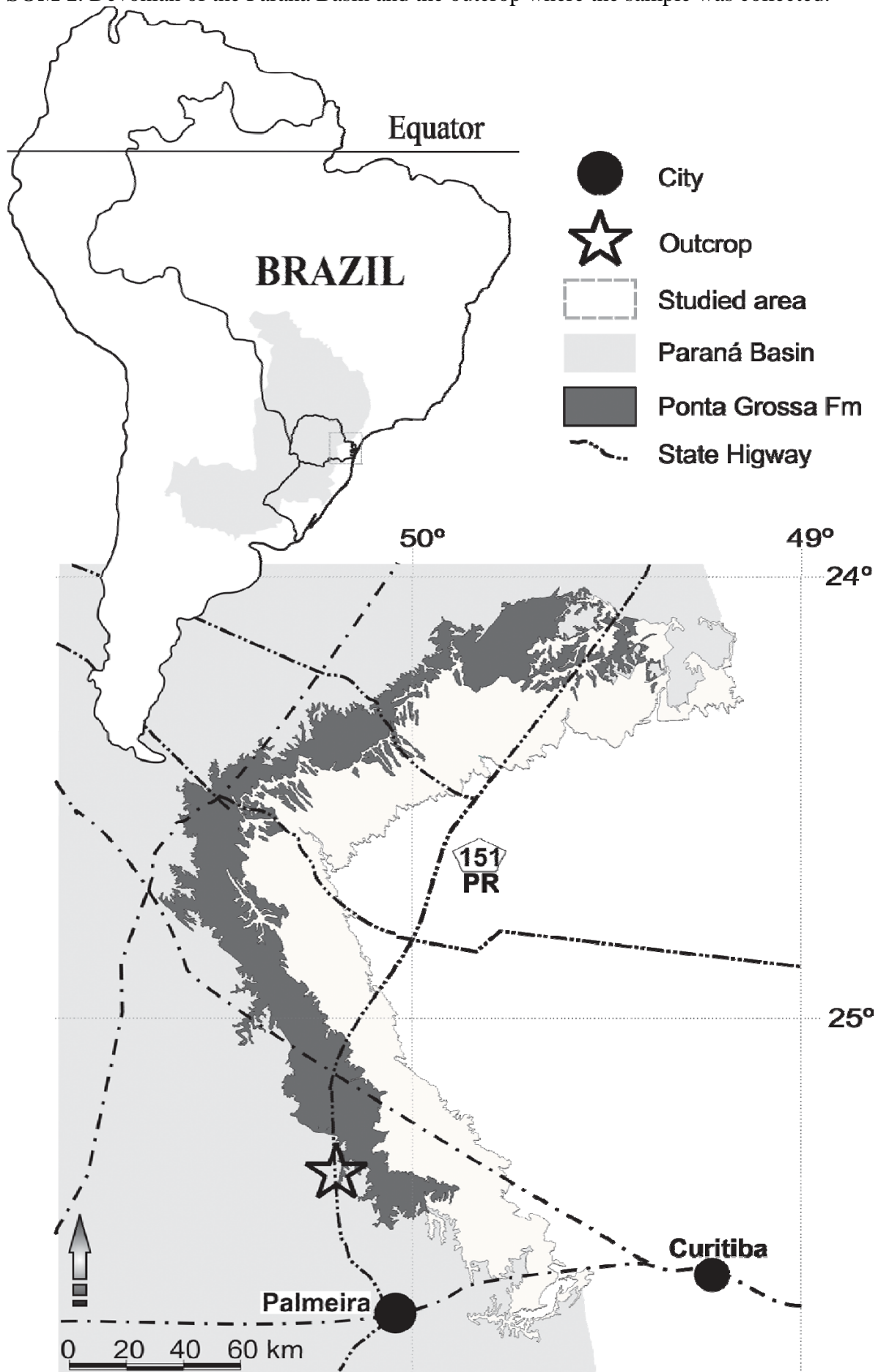
SOM 1. Devonian of the Paraná Basin and the outcrop where the sample was collected.
