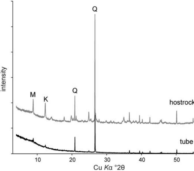
SOM 3. XRD graphic of host rock and studied tubes.
