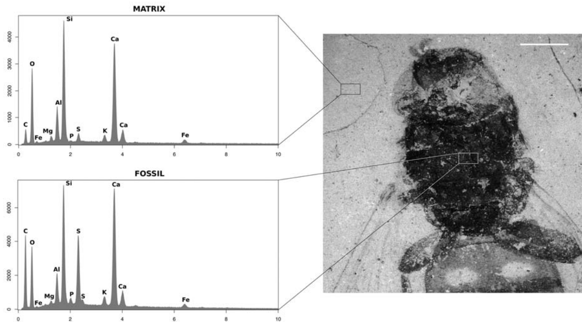
Fig. 1. Energy-dispersive X-ray spectra of the sediment matrix and of material from the thorax of Oligopipiza quadriguttata gen. nov., sp. nov., Rupélian, Céreste, holotype S01, with the locations of the analyzed material indicated. Abscissa in keV, ordinate in cps/eV. Scale bar = 1 mm.
