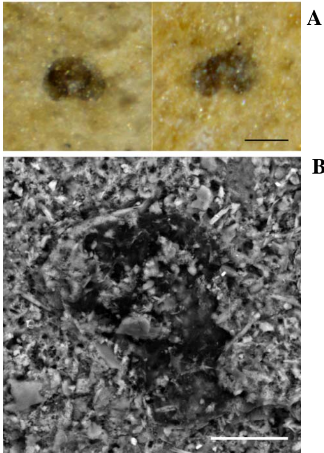
Fig. 2. Fossil pollen grains found on the matrix. Rupelian, Céreste. A. Two fossil pollen grains found on matrix (optical microscopy). B. Pollen grain of a Pinaceae sp. (ESEM, BSE). Scale bars = 40 \mu\text{m} (A), 20 \mu\text{m} (B).
