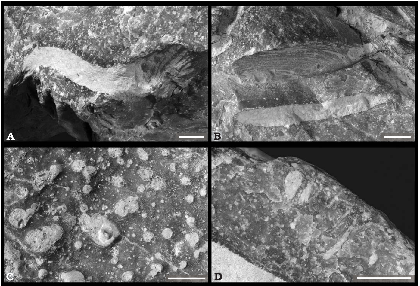
Fig. 4. Close-ups of the bored Densastroma pexisum stromatoporoid (positions indicated by dashed lines in Fig. 3). A. Undulating course of a deeply penetrating Osprioneides kampto Beuck and Wisshak, igen. et isp. nov. in longitudinal section. B. Two unroofed O. kampto Beuck and Wisshak, igen. et isp. nov. specimen, one of which showing the growth increments of the host stromatoporoid on the boring walls where the micritic infill is eroded. Boring direction was from the eroded aperture at the right towards the left hand side. C. The densely pitted outer surface of the stromatoporoid showing circular apertures of Trypanites and Palaeosabella of various size. D. The nearby fracture surface, exposing longitudinal to oblique sections of small Trypanites and Palaeosabella borings. Scale bars 10 mm.
