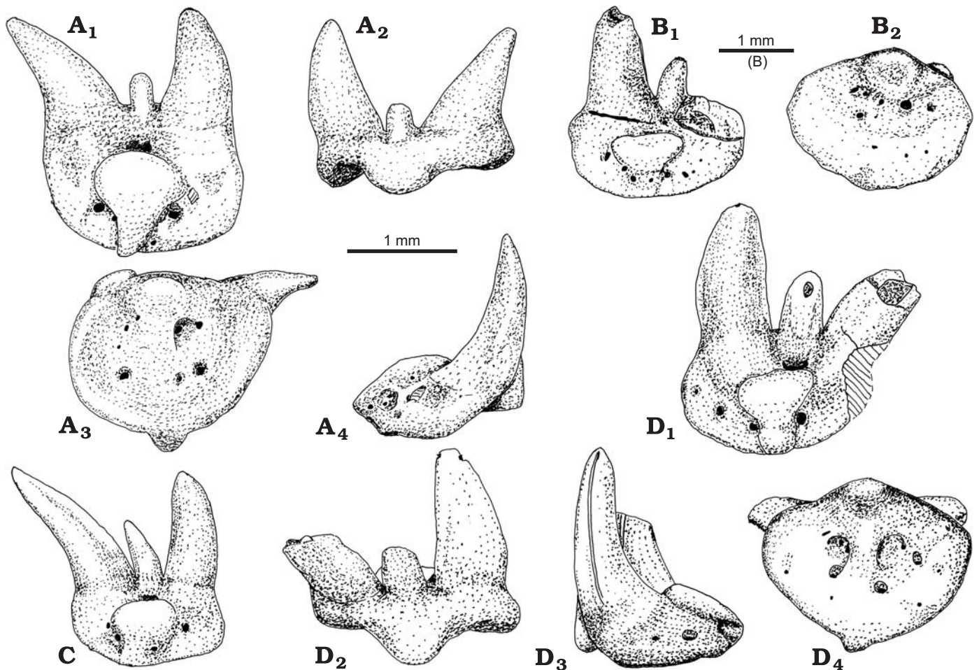
Fig. 7. Diplodoselelchid chondrichthyan Orthacanthus donnelljohnsi sp. nov., juvenile lateral teeth, Lower Pennsylvanian, Black Prince Limestone, Swisshelm Mountains, Arizona. A. UAPL 23390; lingual-occlusal (A 1 ), labial (A 2 ), aboral (A 3 ), and anteromedial (A 4 ) views. B. UAPL 23391; lingual-occlusal (B 1 ) and aboral (B 2 ) views. C. UAPL 23392; lingual-occlusal view (matrix prevented other views). D. UAPL 23393; lingual-occlusal (D 1 ), (posterior margin of oral surface covered by matrix), labial (D 2 ), anteromedial (D 3 ), and aboral (D 4 ) views.
