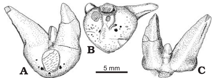
Fig. 5. Diploselachid chondrichthyan Orthacanthus donnelljohnsi sp. nov., adult lateral tooth, UAPL 23383, Lower Pennsylvanian, Black Prince Limestone, Swisshelm Mountains, Arizona; lingual-occlusal (A), aboral (B), and labial (C) views.
