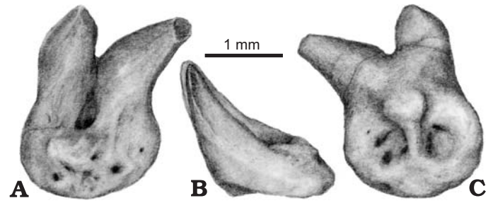
Fig. 4. Diploselachid chondrichthyan Orthacanthus donnelljohnsi sp. nov., adult posterior tooth, UAPL 23387, Lower Pennsylvanian, Black Prince Limestone, Swisshelm Mountains, Arizona; lingual-occlusal (A) anterior (B), and aboral (C) views.
