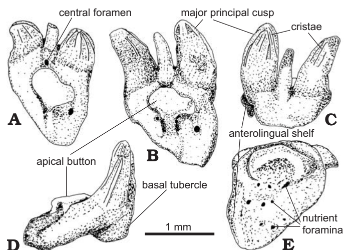
Fig. 12. Xenacanthid chondrichthyan Triodus elpia sp. nov., lateral tooth, holotype, UAPL 23397, Lower Pennsylvanian, Black Prince Limestone, Swisshelm Mountains, Arizona; occlusal (A), lingual-occlusal (B), labial (C), anteromedial (D), and aboral (E) views; note the lingual extension on the apical button in B.
