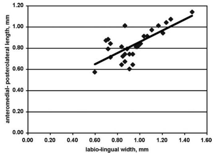
Fig. 13. Scatter diagram of Triodus elpia sp. nov. tooth base dimensions.
