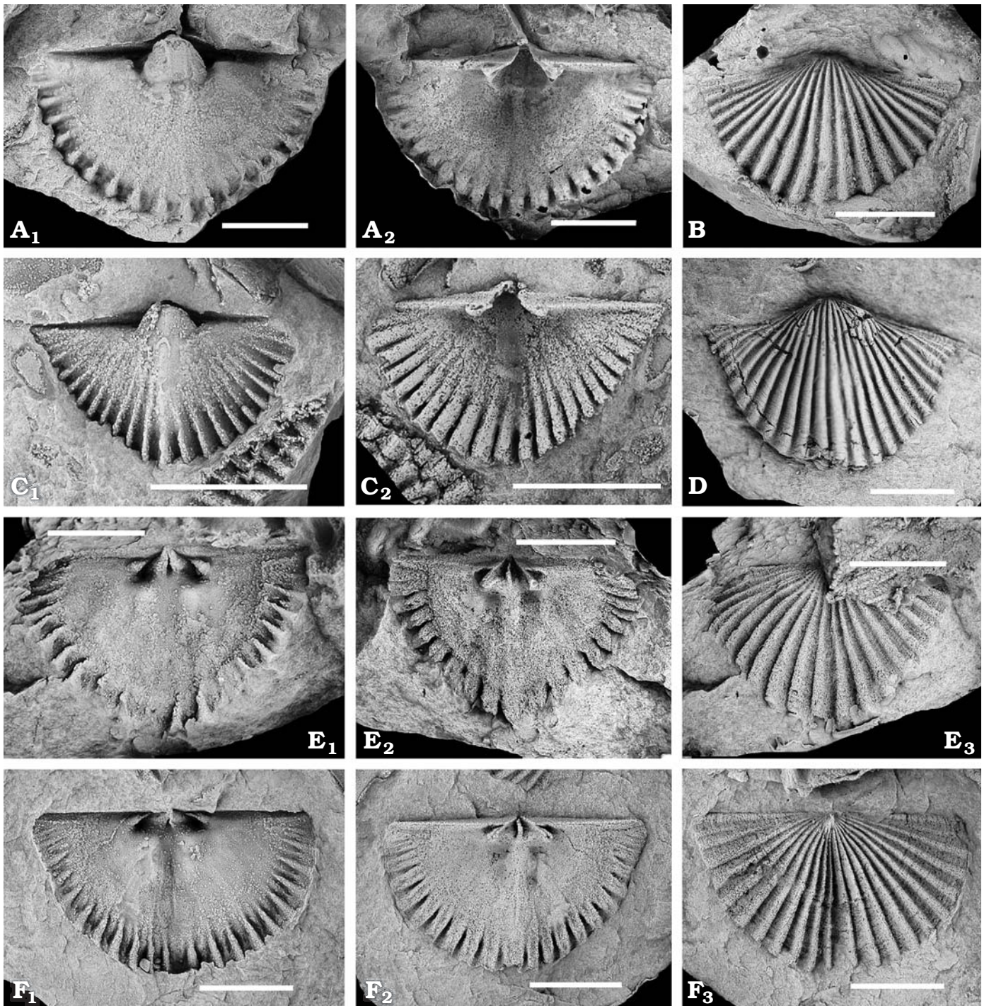
Fig. 8. Orthid brachiopod Paralenorthis lolae Reyes-Abril and Villas sp. nov. A. Holotype, MGM-6121-O, internal mould (A 1 ) and latex cast of interior (A 2 ) of ventral valve. B. MGM-6133-O, latex cast of exterior of ventral valve. C. MGM-6129-O, internal mould (C 1 ) and latex cast of interior (C 2 ) of ventral valve. D. MGM-6135-O, latex cast of exterior of ventral valve. E. MGM-6143-O, internal mould (E 1 ) latex cast of interior (E 2 ) and latex cast of exterior (E 3 ) of dorsal valve. F. MGM-6158-O, internal mould (F 1 ), latex cast of interior (F 2 ) and latex cast of exterior (F 3 ) of dorsal valve. Scale bars 5 mm.
