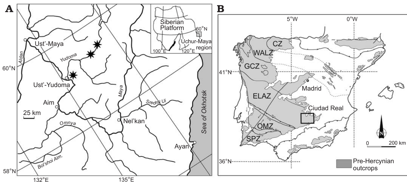
Fig. 1. Maps indicating studied localities. A. Map of Uchur-Maya region showing reference sections of the Yudoma River: 1, Nuuchchalakh; 2, Kyry-Ytyga; 3, Ust'-Yudoma ( Sovorovella and Majaella locality). Inset map indicates location within Siberian Platform. B. Pre-Hercynian outcrops and tectonostratigraphic zones of Iberian Peninsula. Valdelacasa, Ibor, Navalpino, and Abenójar anticlines are outlined. Zones: CZ, Cantabrian; ELAZ, East Lusitanian-Alcudian; GCZ, Galician-Castilian; OMZ, Ossa-Morena; SPZ South Portuguese; WALZ, West Asturian-Leonese.
