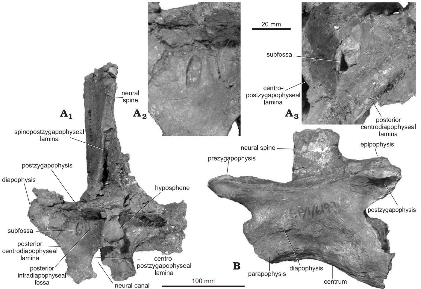
Fig. 10. Vertebrae of the Spion Kop sauropod from the Lower Jurassic Elliot Formation of South Africa. A. Posterior dorsal vertebra, BP/1/6183a in posterior view (A 1 ). Close-up of left (A 2 ) and right (A 3 ) posterior infradiapophyseal fossae. Note that the right subfossa cannot be seen in A 1 due to the oblique distortion of the specimen. B. Cervical vertebra, ?C3, BP/1/6199 in left lateral view.
