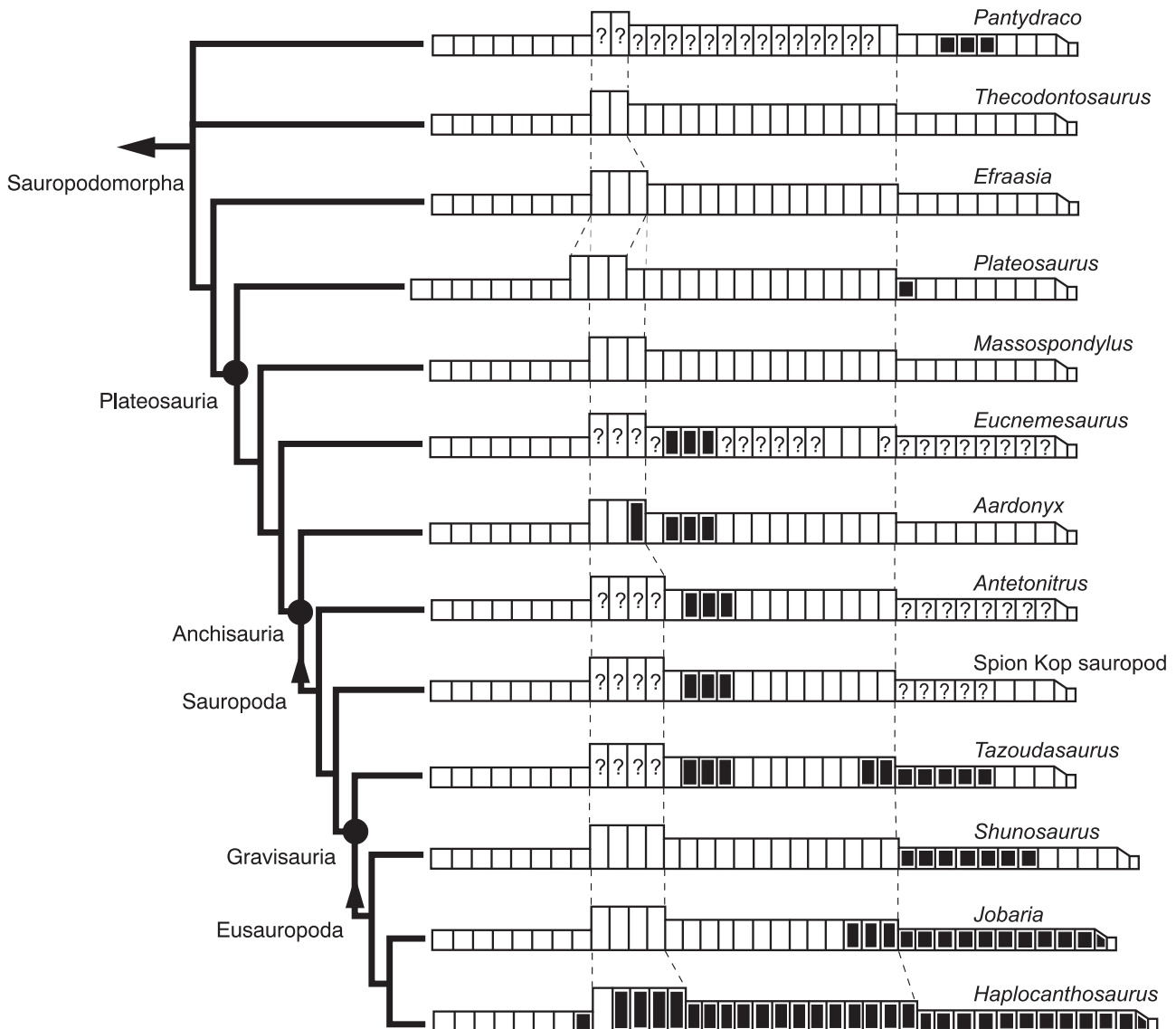
Fig. 12. A phylogenetic diagram showing the distribution of invasive PSP along the vertebral column (the caudal series is truncated) in Sauropodomorpha. Black boxes indicate the presence of pneumatic fossae or invasive infradiapophyseal subfossae. Note that in the case of Plateosaurus PSP is presently known in a single specimen whereas other specimens of same taxon lack it. The phylogeny is based on Yates (2010), with the modification that Eucnemesaurus is placed closer to Anchisauria than Massospondylus is. The position of the Spion Kop sauropod is based on an unpublished analysis (AMY unpublished data). The distributions of PSP in the taxa not directly examined in this study were gleaned from the following sources: Pantydraco (Yates 2003; Wedel 2007), Tazoudasaurus (Allain and Aquesbi 2008), Shunosaurus (Zhang 1988), Jobaria (Serenio et al. 1999), Haplocanthosaurus (Hatcher 1903).
