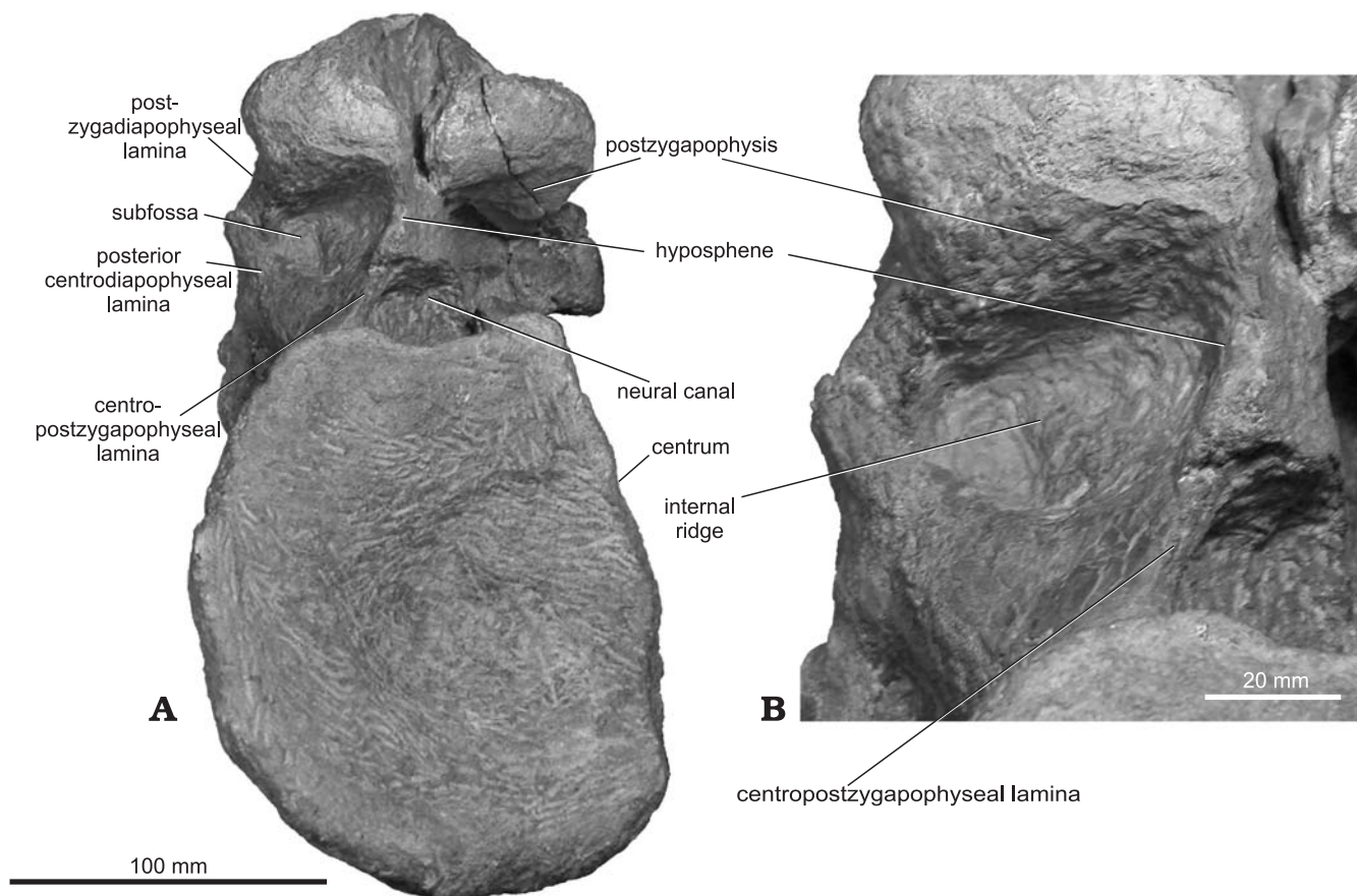
Fig. 11. Posterior dorsal vertebra of the basal sauropodomorph Camelotia borealis Galton, 1985, NHM R.2873 from the Upper Triassic Westbury Formation of Somerset, England. A . Posterior view. B . Close-up of left posterior infradiapophyseal fossa.
