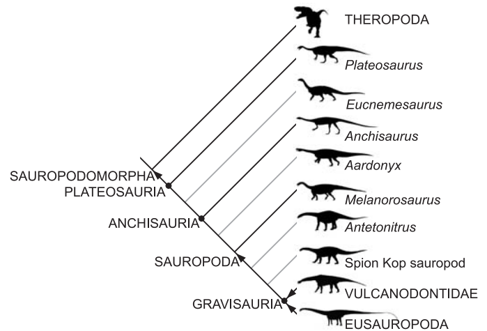
Fig. 2. A simplified cladogram of sauropodomorph dinosaurs indicating the relative positions of various anchor taxa, or their inclusive clades, other taxa discussed in the paper and the higher-level taxonomy that is used. Dots represent node-based taxa, arrows represent stem-based taxa.
