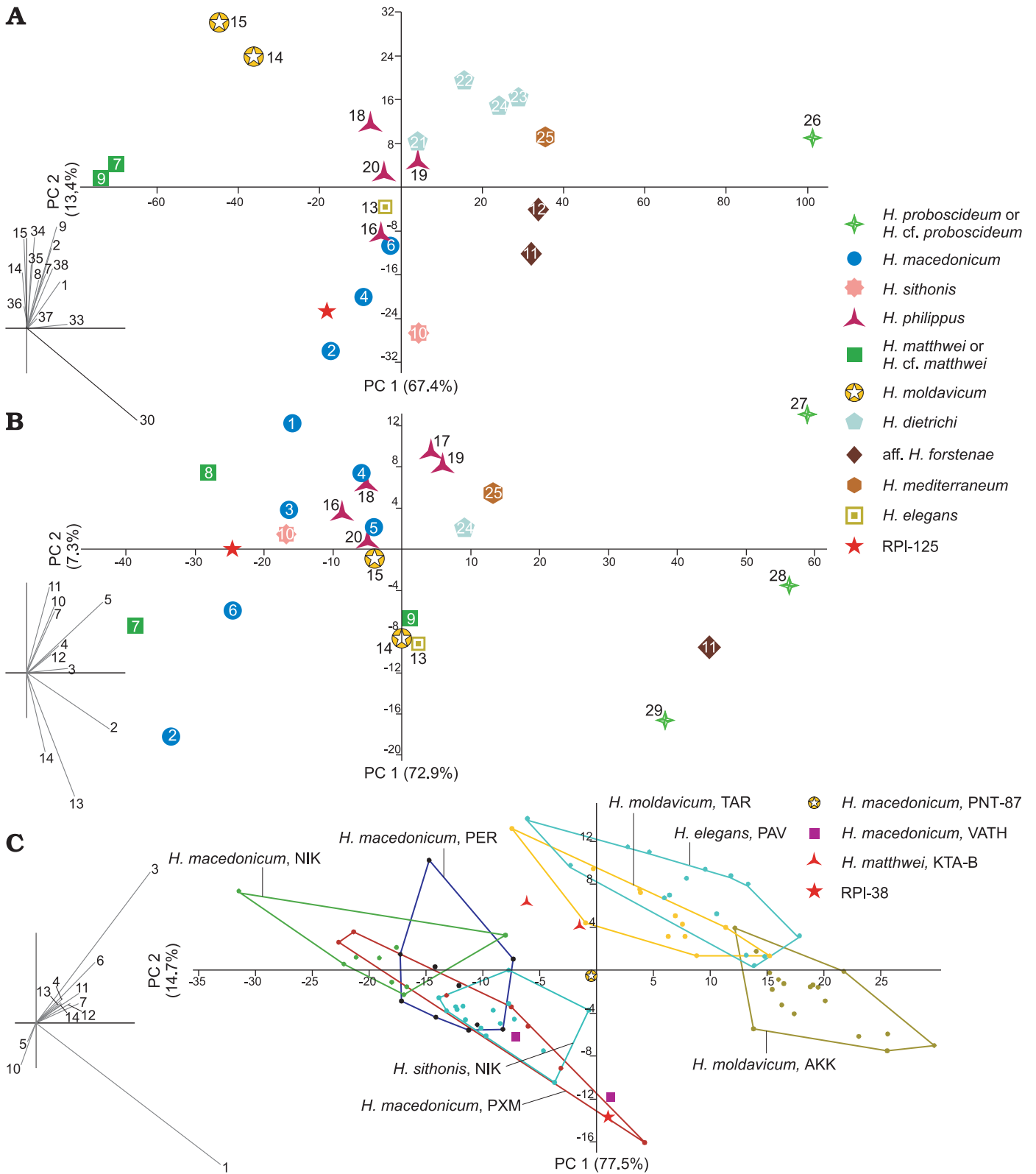
Fig. 4. Principal component analysis of the skull (A), mandible (B), and third metatarsal (C) of the RPI small-sized hipparion in comparison with other small-sized forms of Eurasia, indicating its strong size-similarities with Hipparion macedonicum . As the available specimens are fragmentary, lacking measurements the mean cranial dimensions for each locality are used. The used variables (various measurements of the skull, mandible and Mt III ) and their influence to the distinction of the specimens is given in the left part of the diagrams. The convex hulls indicate the allocation of the measurements in the space for its sample. Hipparion dietrichi , Hipparion mediterraneum , and Hipparion proboscideum or Hipparion cf. proboscideum are used as comparative samples. Hipparion macedonicum : 1, NKT; 2, NIK; 3, RZO; 4, PXM; 5, VATH; 6, PER. Hipparion matthewi : 7, Samos (unknown locality), holotype; 8, KTA-B. Hipparion cf. matthewi : 9, MTLA. Hipparion sithonis : 10, NIK. aff. Hipparion forstenae : 11, MTLA; 12, Samos Q1. Hipparion →
