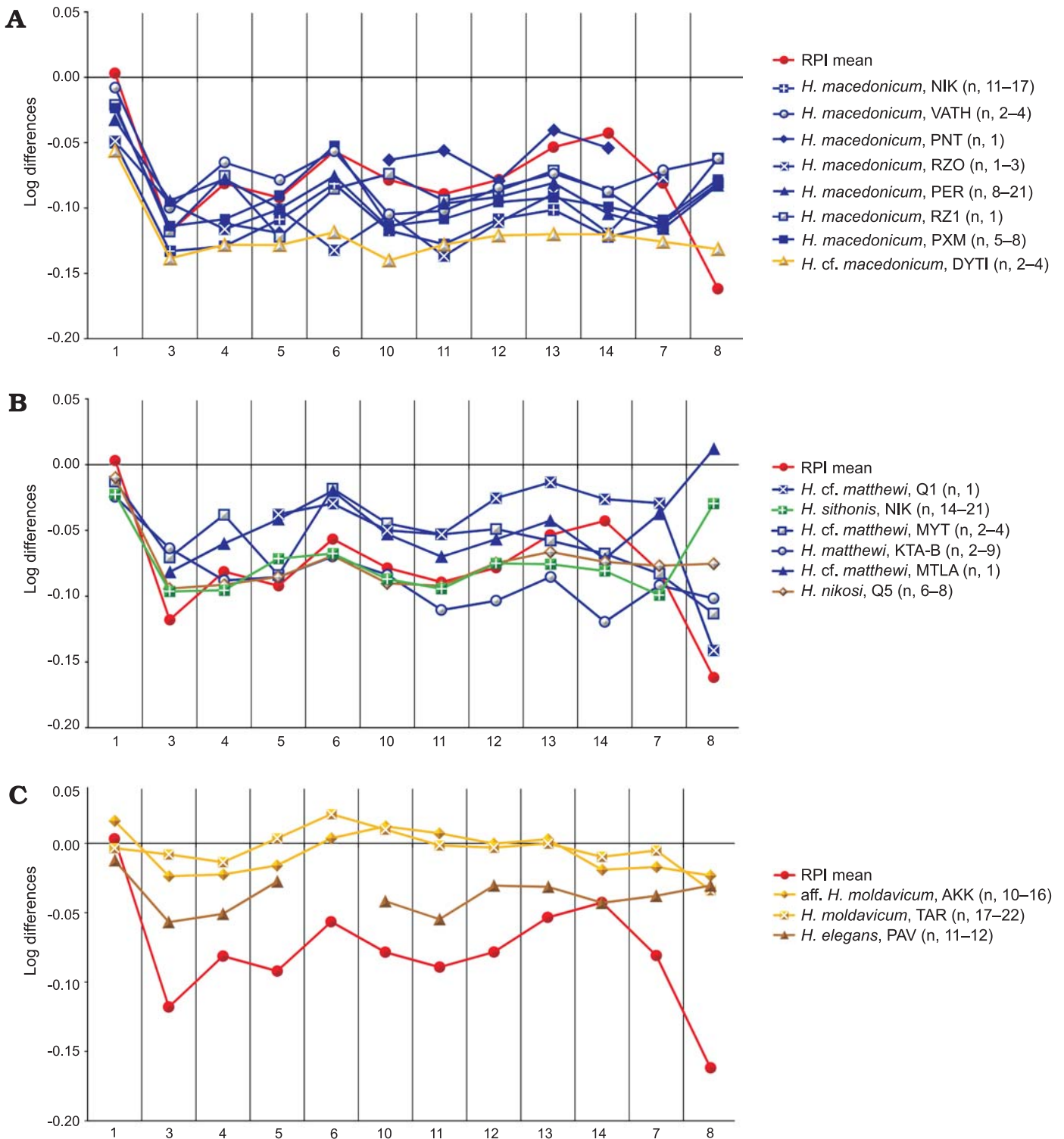
Fig. 7. Logarithmic ratio diagram comparing the RPI third metatarsal with Hipparion macedonicum and other small-sized hipparions from various localities. Hipparion mediterraneum from Pikermi (Koufos 1987a) is used as standard of comparison. The metrical data for the hipparions from Greek localities and AKK are from my own archive; those for Hipparion moldavicum from TAR and Hipparion elegans from PAV are taken from http://www.vera-eisenmann.com .
