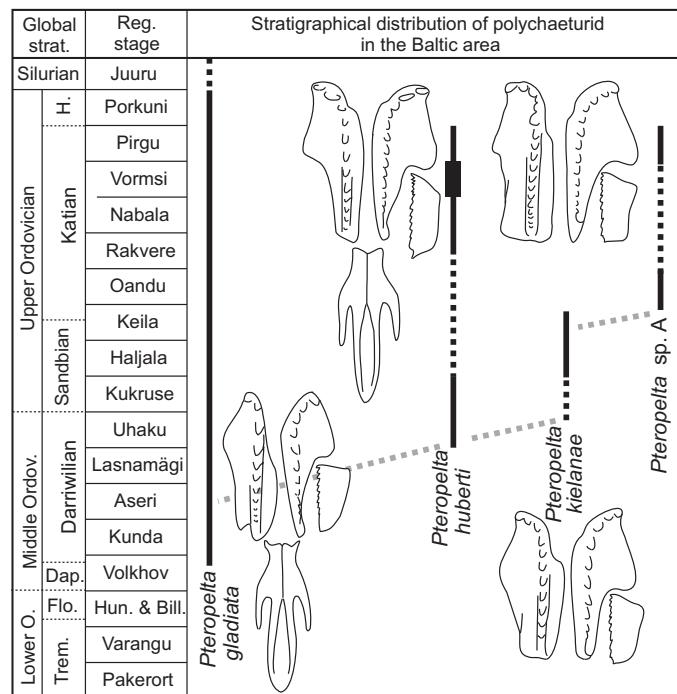
Fig. 3. Stratigraphical distribution of polychaeturids in the Baltic region and also showing the tentative phylogenetic relationship between the different species. The stratigraphical chart is slightly modified from Nölvak et al. (2006). Abbreviations: Dap., Dapingian; Flo., Floian; H., Hirnantian; Hun. & Bill., Hunneberg and Billingen; Reg., regional; Trem., Tremadocian.
