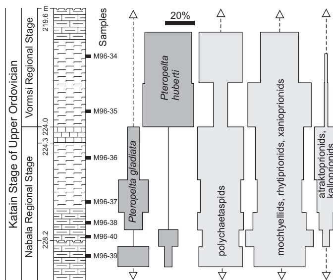
Fig. 5. Pattern of relative abundance (%) of polychaetoid polychaetes Pteropelta gladiata and Pteropelta huberti in the Laeva 18 drill core, central Estonia. The counts are based on a total of 572 posterior maxillae (MI), of which 147 belong to polychaetoid. Arrow heads indicate that the ranges continue beyond the interval shown.
