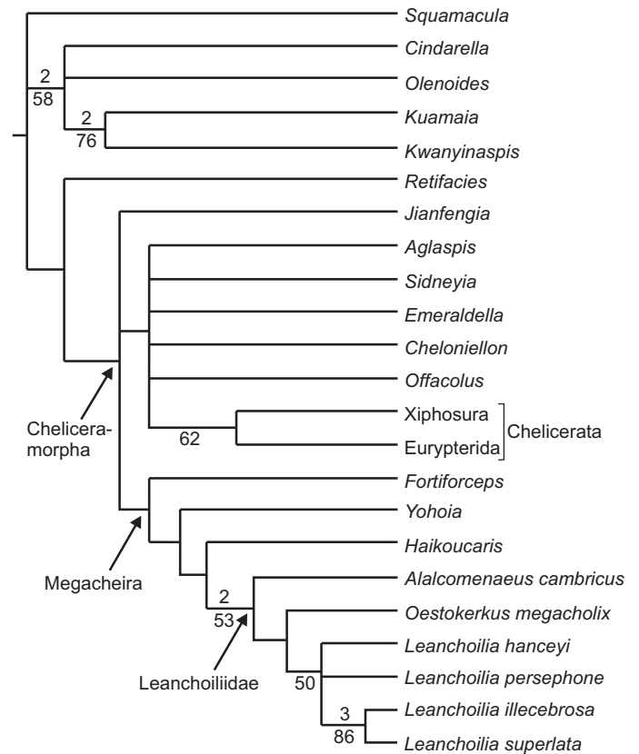
Fig. 8. Strict consensus of 14 shortest cladograms (77 steps) based on character data in Table 1. Numbers above nodes are Bremer support; those below nodes are jackknife frequencies >50%. Chelicera-morpha corresponds to a clade with the same composition in Cotton and Braddy (2004).
