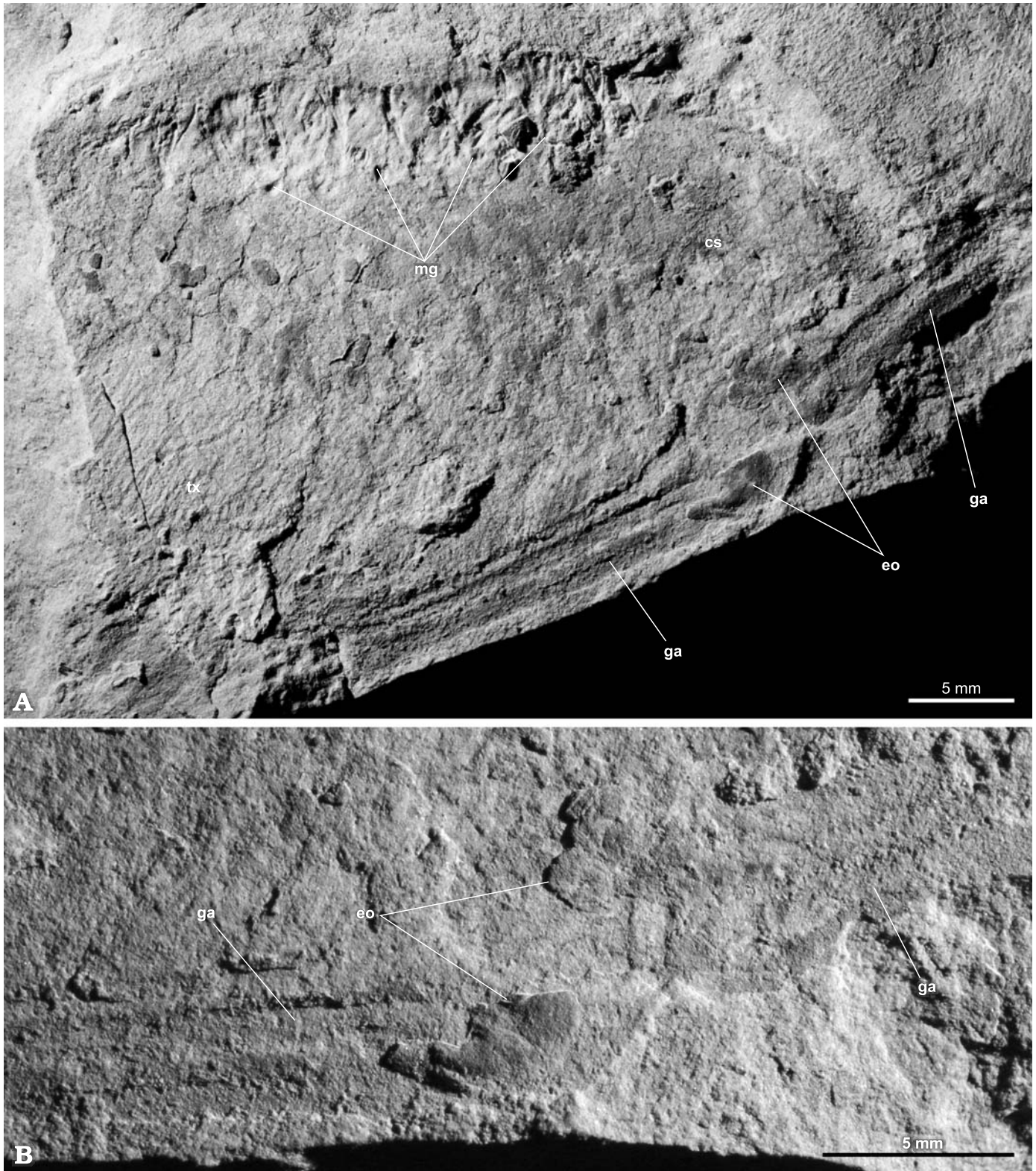
Fig. 6. Leanchoiliid megacheiran arthropod Oestokerkus megacholix gen. et sp. nov. SAM P45168. A. head and anterior part of trunk. B. Detail of spinose projections of great appendages and excretory organs (sensu Bruton and Whittington 1983). Abbreviations: cs, cephalic shield; eo, excretory organ; ga, great appendage; mg, midgut glands; tx, trunk exopods.
