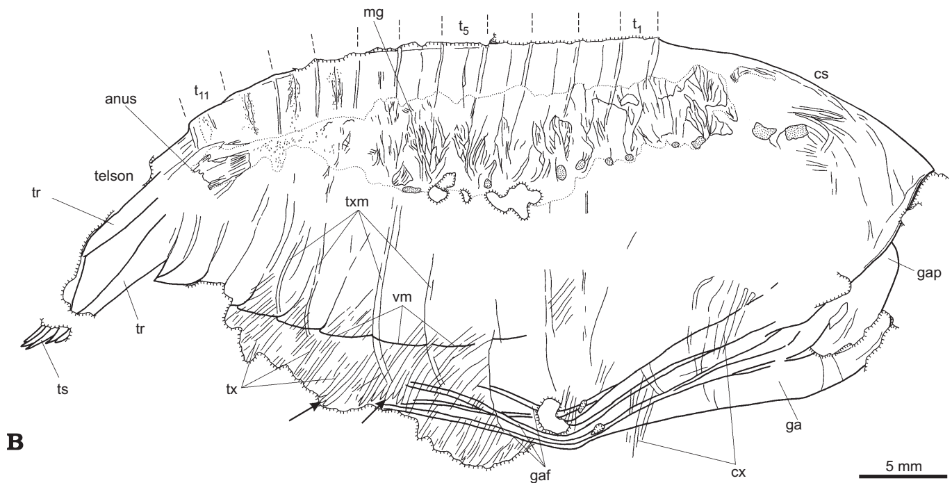
Fig. 2. Leanchoiliid megacheiran arthropod Oestokerkus megacholix gen. et sp. nov. Holotype SAM P43631a. A. Photograph. B. Interpretative camera lucida drawing. Arrows indicate tips of trunk exopod setae. Abbreviations: cs, cephalic shield; cx, cephalic exopods; ga, great appendage; gaf, great appendage flagellum; gap, peduncle of great appendage; mg, midgut glands; t1, tergite of trunk segment 1; tr, reinforcing ridges on telson; ts, telson marginal spines; tx, trunk exopods; txm, trunk exopod lobe margins; vm, ventral margin of tergites. Boundaries between trunk tergites indicated by dashed lines above dorsal margin.
