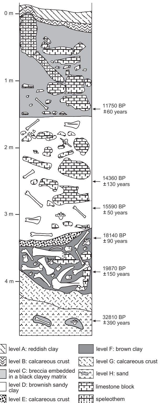
Fig. 2. Stratigraphic section and radiocarbon dates for the locality of Kiputz IX.
