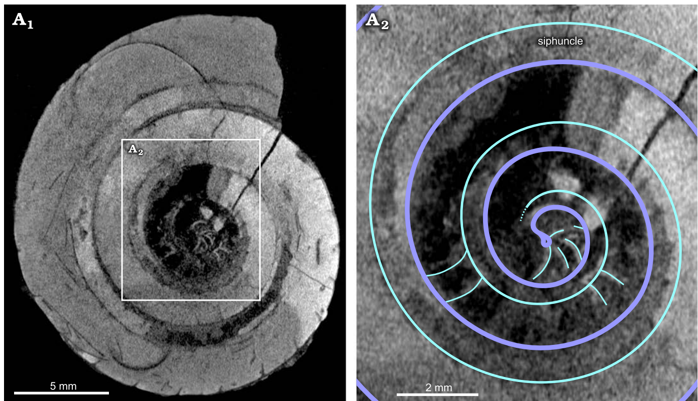
Fig. 6. Tarphyceratid cephalopod Trocholites chaloupkai sp. nov. from Praha-Štěrboholý, central Bohemia, Czech Republic, upper part of the Zahořany Formation (lower Katian, Upper Ordovician). A. Holotype NM L 63626, detail of apicalmost part of the phragmocone (A 1 ) and drawing (A 2 ) indicating line of contact of whorls, position of siphuncle, position of (partly fragmented) septa and shape of initial chamber and umbilical window.
