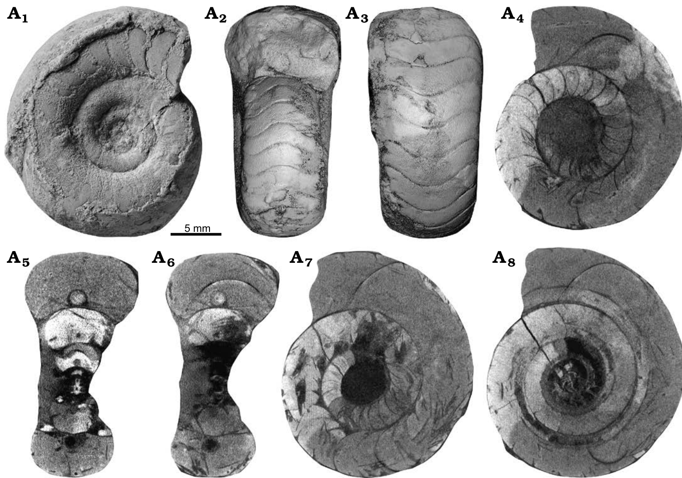
Fig. 5. Taphyceratid cephalopod Trocholites chaloupkai sp. nov. from Praha-Štěrboholy, central Bohemia, Czech Republic, upper part of the Zahořany Formation (lower Katian, Upper Ordovician). Holotype NM L 63626, optical microscope photograph of whitened specimen in lateral view (A 1 ); micro-CT images showing frontal (A 2 ) and ventral (A 3 ) views, note ventral lobe of suture line; virtual longitudinal sections in sagittal plane showing partly preserved septa in last (A 4 ) and penultimate (A 5 ) whorls; virtual longitudinal section in median plane (A 6 ) showing the siphuncle and the earliest whorl of the phragmocone; virtual transverse sections in slightly eccentric (A 7 ) and central (A 8 ) planes documenting whorl profile shape and siphuncle.
