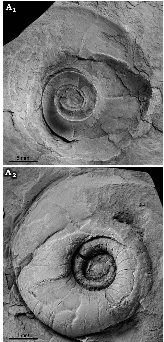
Fig. 4. Tarphyceratid cephalopod Trocholites fugax Babin and Gutiérrez-Marco, 1992, from Březová Hůrka near Starý Plzeň, central Bohemia, Czech Republic, Dobrotivá Formation (upper Middle–lower Upper Ordovician). A. NM L 63625a, b, counterpart (A 1 ) and part (A 2 ).
