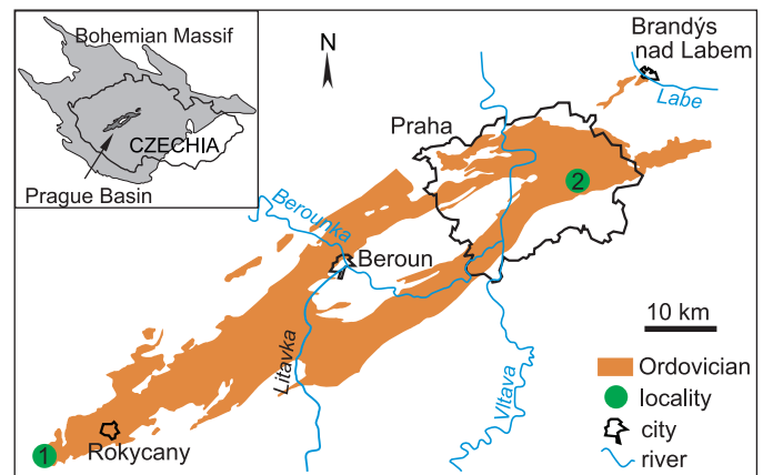
Fig. 1. Map of Ordovician rocks of the Prague Basin and position of the localities, from which the two studied specimens originate: Locality 1, Březová Hůrka near Starý Plzeň; Locality 2, Praha-Štěrboholy. Modified from Manda (2008).
